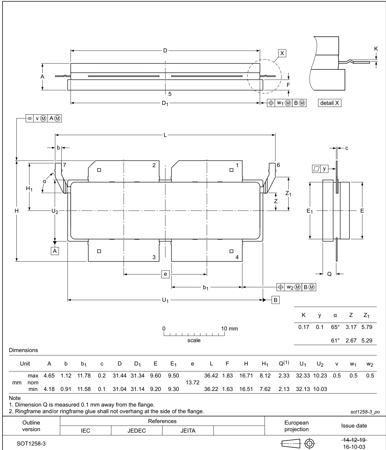
Fig 12. Package outline SOT1258-3
